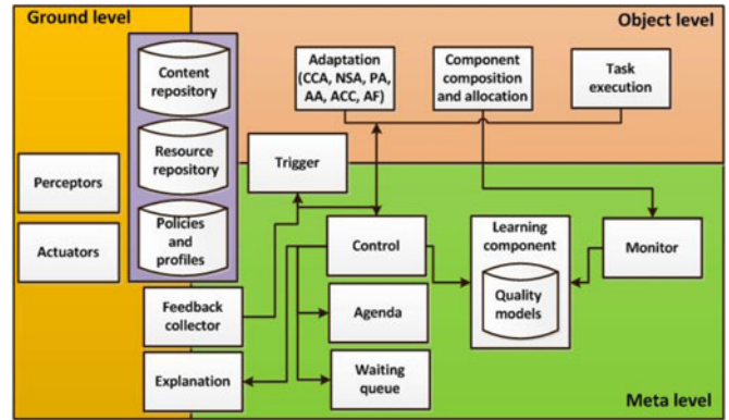
Fig. 5. Reference architecture for adding meta-level functionality to ubiquitous learning systems (modified from Gilman and Riekkii [17]).
