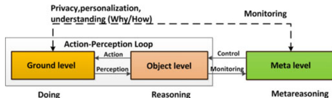
Fig. 4. Metareasoning concept visualization, modified from Cox and Raja [57] and Gilman and Riekkki [17].
