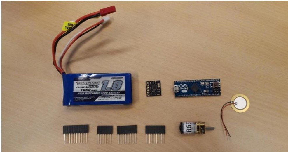
Figure 2. Initial components given to the students (top from left to right: battery, gyro and accelerometer board, Arduino Micro board, and piezo element; bottom: four types of connectors and motor)
